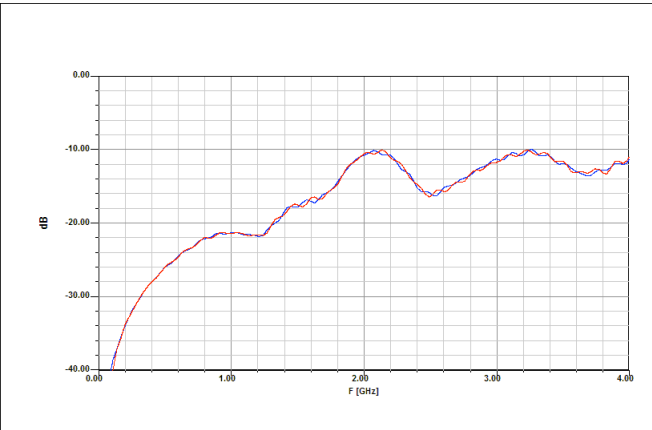
Isolation
