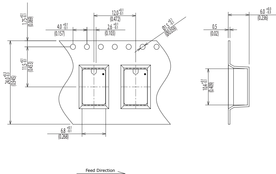
Details of the part A
